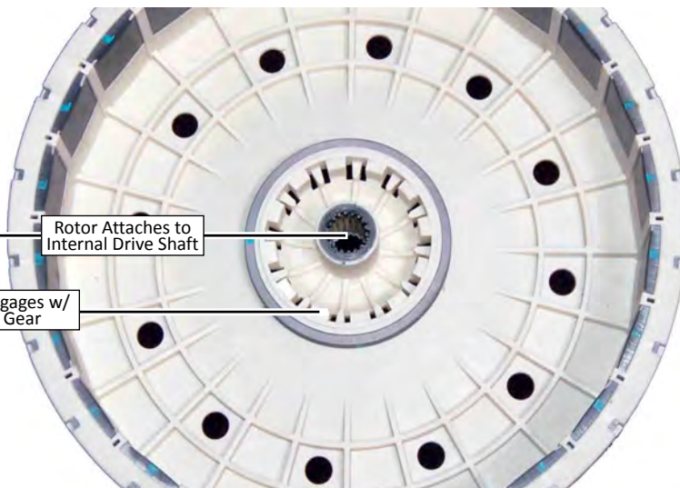
Figure 5 - Rotor
