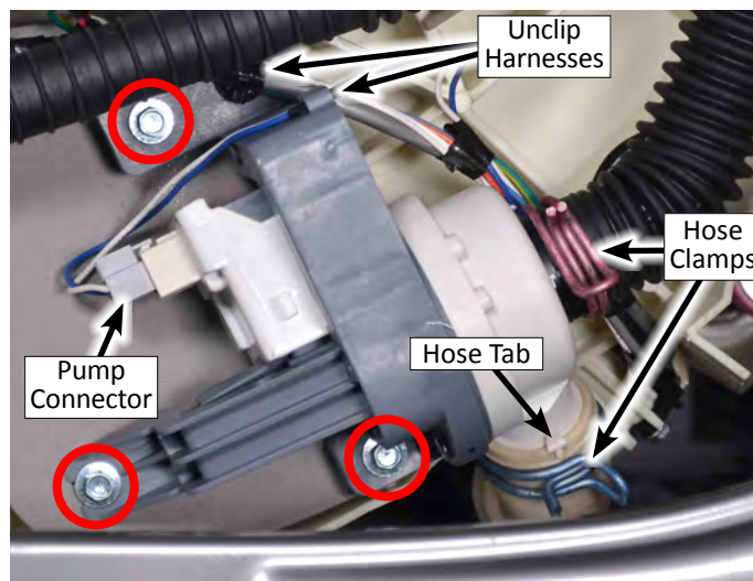
Figure 2 - Drain Pump
