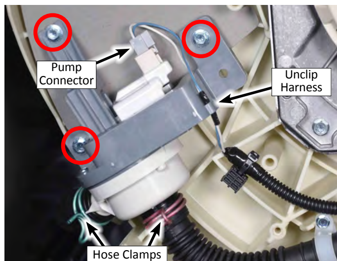
Figure 3 - Recirculation Pump
