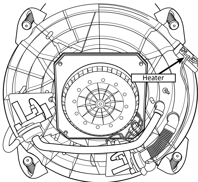
Figure 1 - Heater Location
