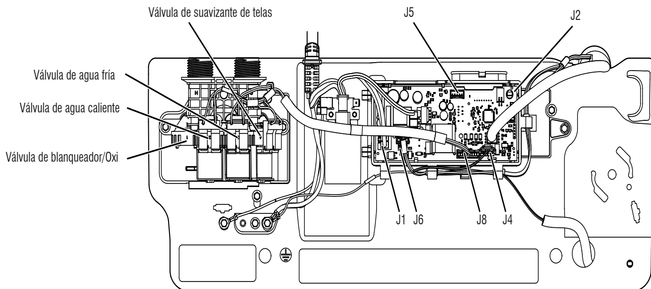
Figura 7: Control principal (ACU)
