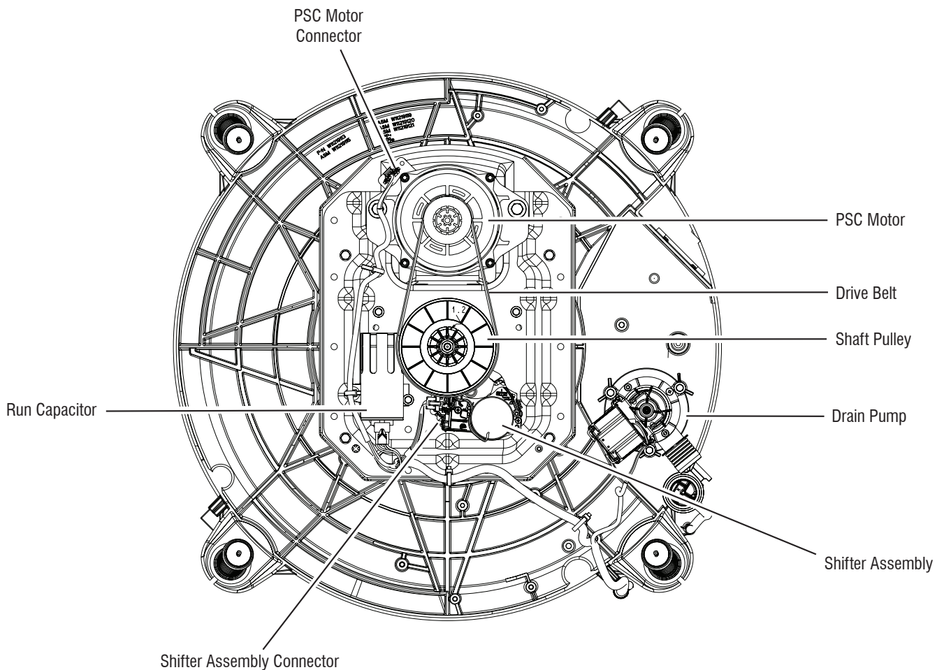
Figure 8 - Bottom View - PSC
