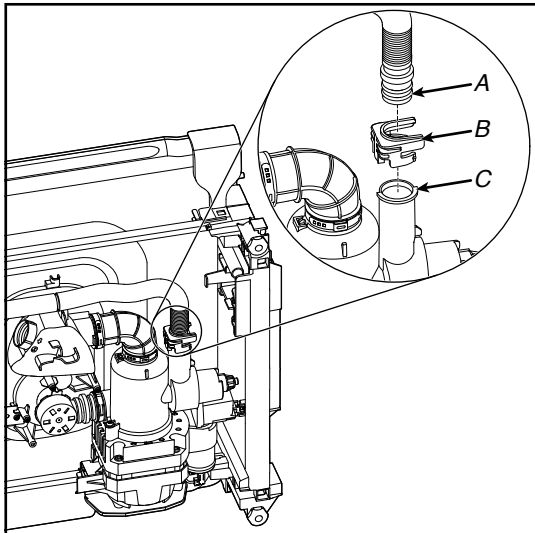
A. Drain Pump Port B. Plastic Hose Retainer C. Drain Pump Hose
